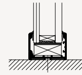
FLOOR CONNECTION
