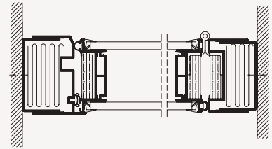
WALL CONNECTION
