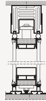
CEILING AND FLOOR CONNECTION
