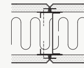
GYPSUM / GYPSUM CONNECTION
