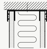
CEILING CONNECTION
