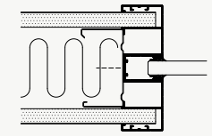
GYPSUM / DEKO FG CONNECTION
