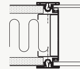
GYPSUM / GLASS CONNECTION
