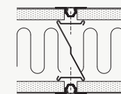
GYPSUM / GYPSUM CONNECTION
