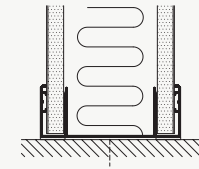
FLOOR CONNECTION
